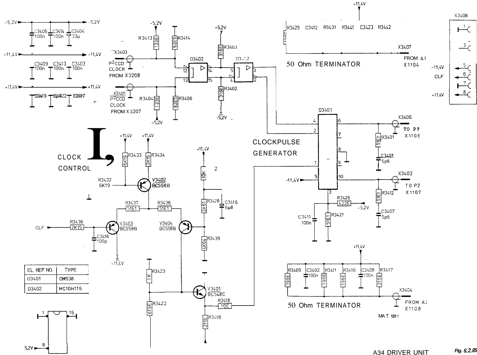
A34 DRIVER UNIT
