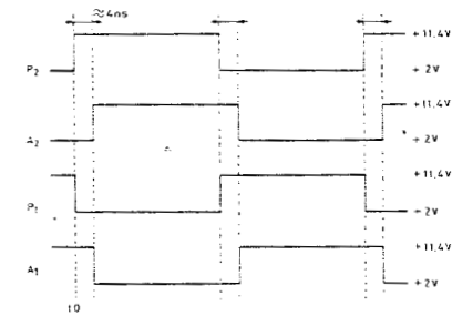
Fig. 6.2.50. Timing clock signals
