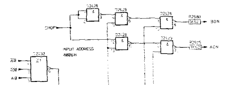
CHOPPER DECODING
