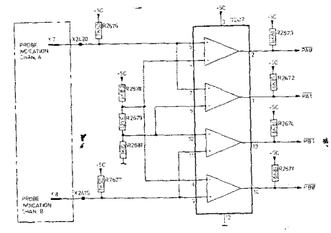
PROBE INDICATION CIRCUIT
