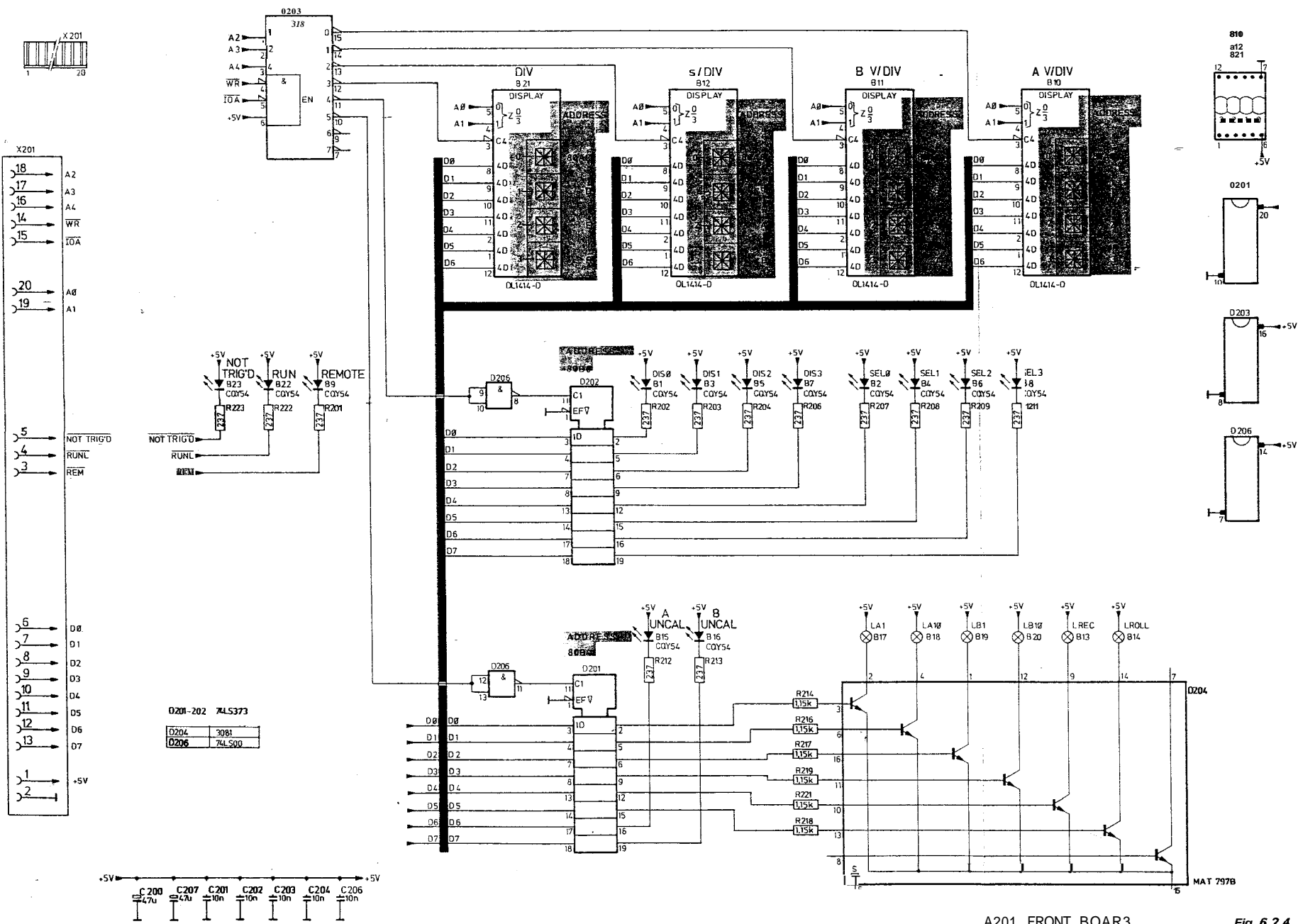
A201 FRONT BOAR3
