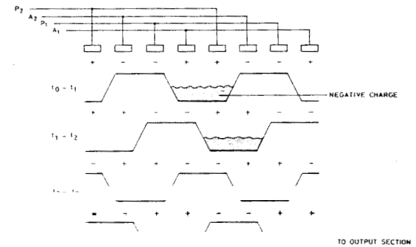
Fig. 6.2.51. Displacement of a negative charge as a function of the clock voltages
